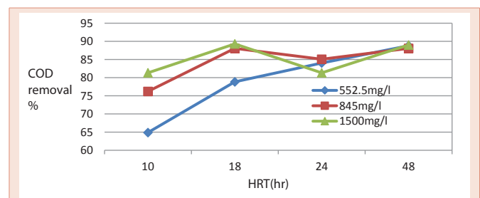
Figure 3: COD removal rate at different HRT at different COD loads of ethylene glycol.
