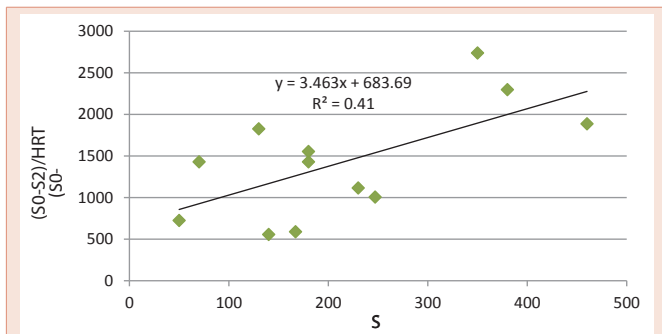
Figure 4: Correlation between Monod model and experimental pilot.
