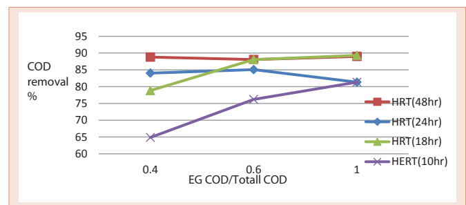
Figure 2: COD removal rates for the MBBR system at different HRT.
