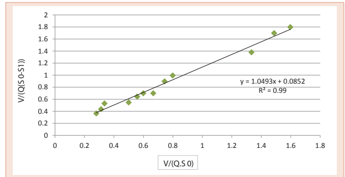
Figure 5 Correlation between Stover-Kincannon model and experimental pilot.
