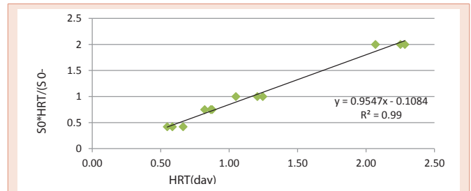
Figure 6 Correlation between Grau second-order substrate removal and experimental pilot.
