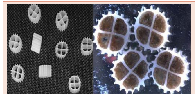
Figure 1: Carrier elements and biofilm formation in the reactor.
